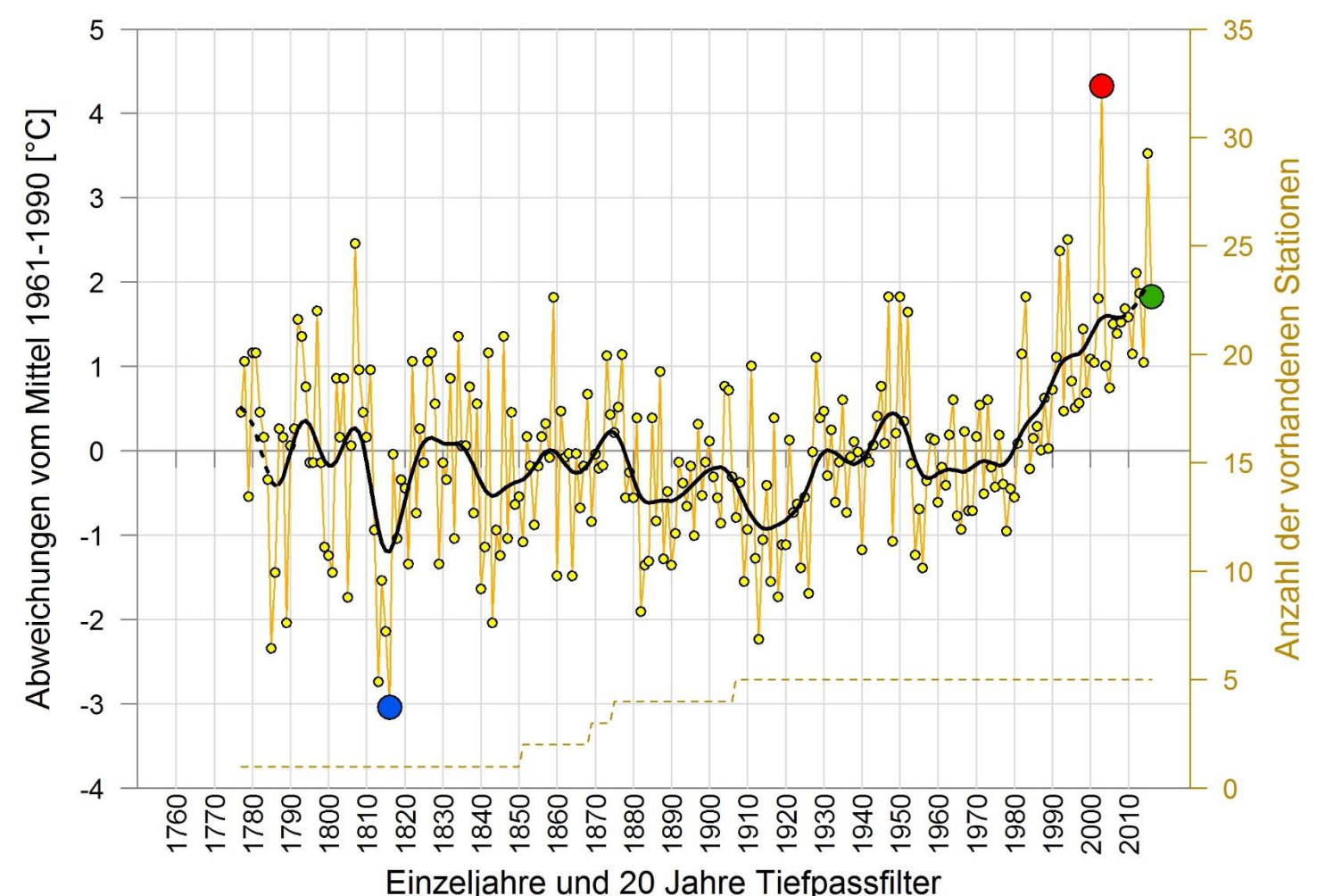
SOMMERMITTELTEMPERATUR 1777 - 2016 REGION WEST
